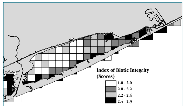
Figure 5. Distribution of IBI scores for East Matagorda Bay (1982-2000).
