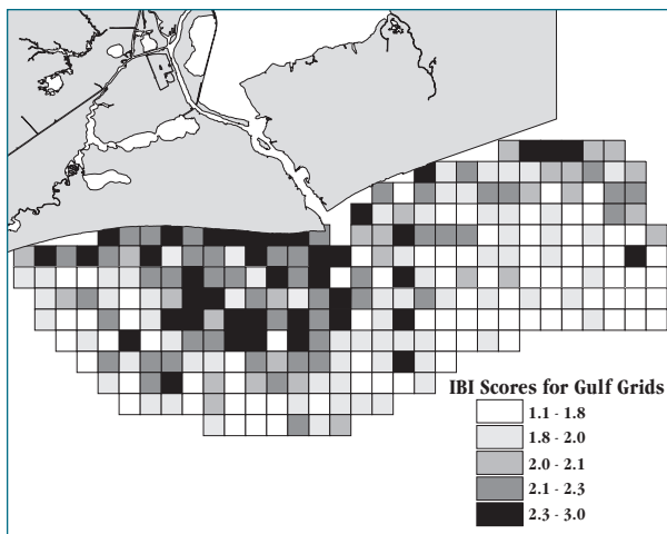
Figure 11. IBI scores for Gulf grids at Sabine Pass.
