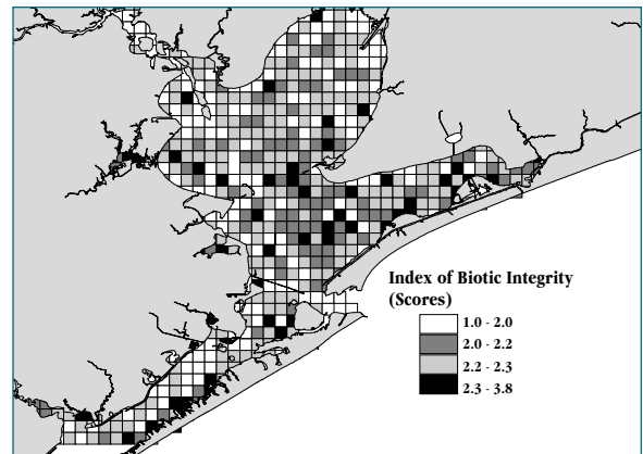
Figure 3. Distribution of IBI scores for Galveston Bay (1982-2000).
