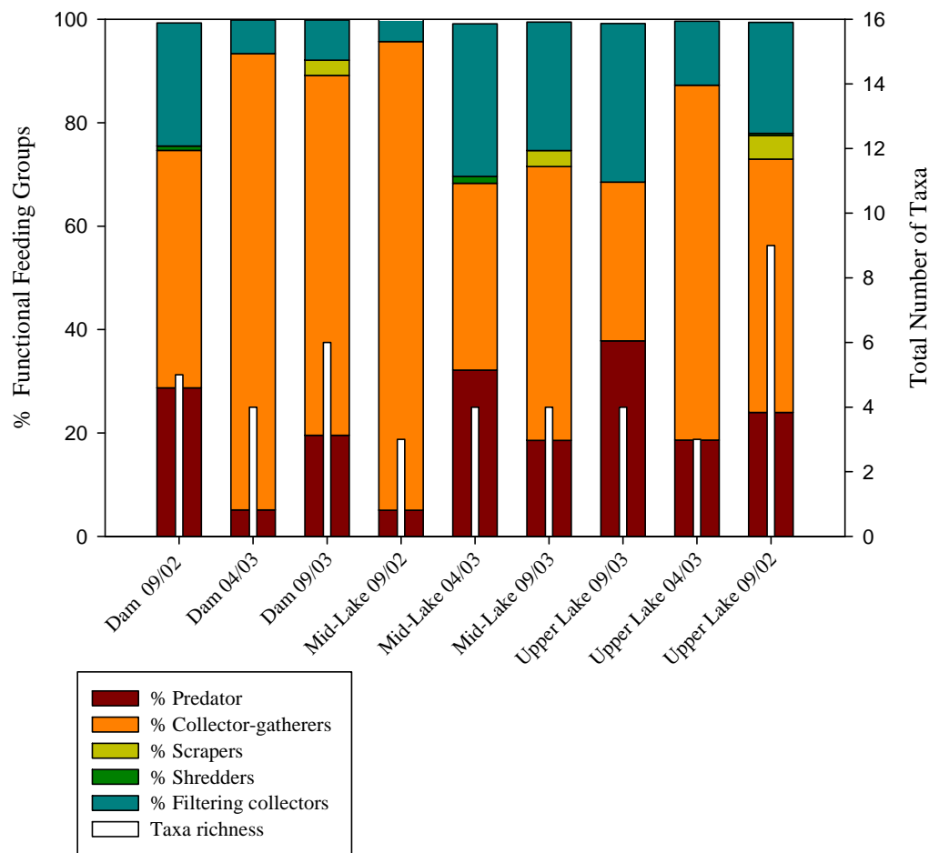
Figure 3. Lake Mexia benthic macroinvertebrate dredge sample data.
