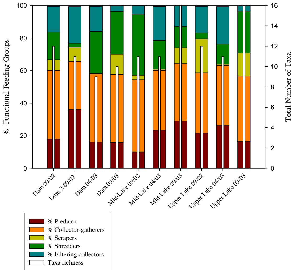
Figure 4. Lake Mexia benthic macroinvertebrate vegetation sample data.
